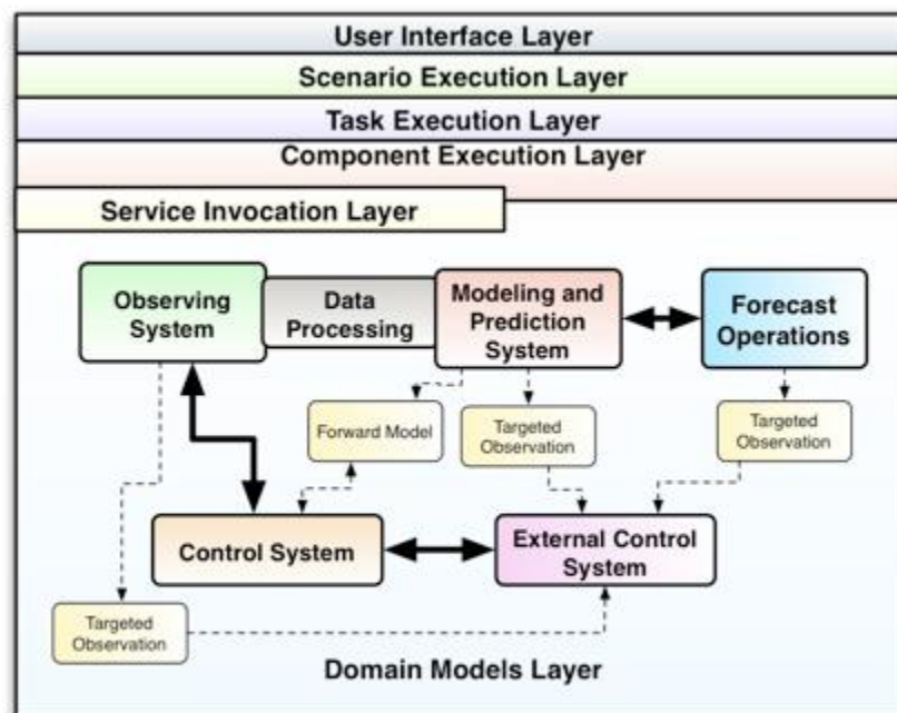
Fig. 1 - Sensor Web Simulator Architecture
