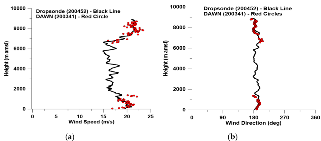
Figure 9. DAWN-dropsonde comparison of wind speed (a) and wind direction (b) for a convectively active case on 21 June 2017 ~200400Z.
