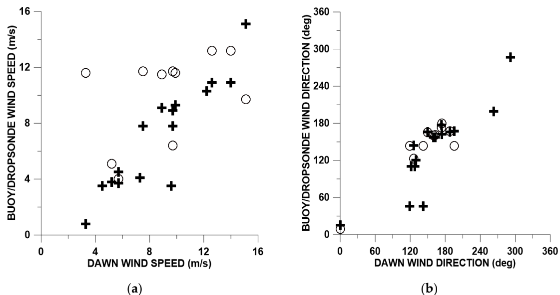
Figure 12. Scatterplots of the DAWN-buoy (+) and DAWN-dropsonde (○) comparisons for wind speed (a) and wind direction (b) during CPEX missions flying over or near NDBC buoys.
