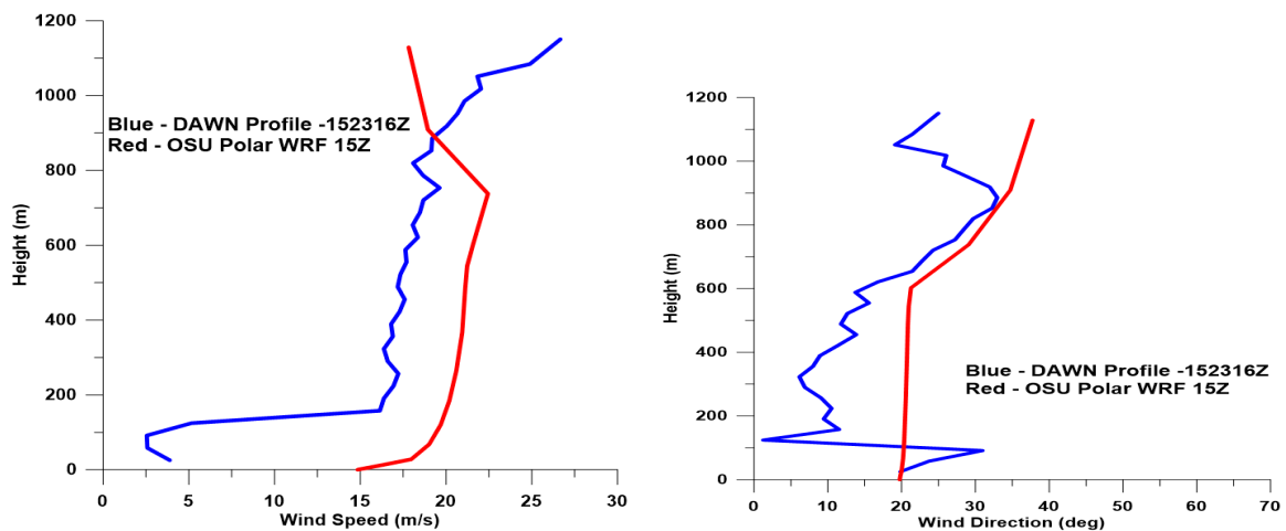
Figure 19. DAWN and model profiles of wind speed (left) and wind direction (right) near 152316Z on 31 October 2014 for the middle of leg 3 east of the tip.
