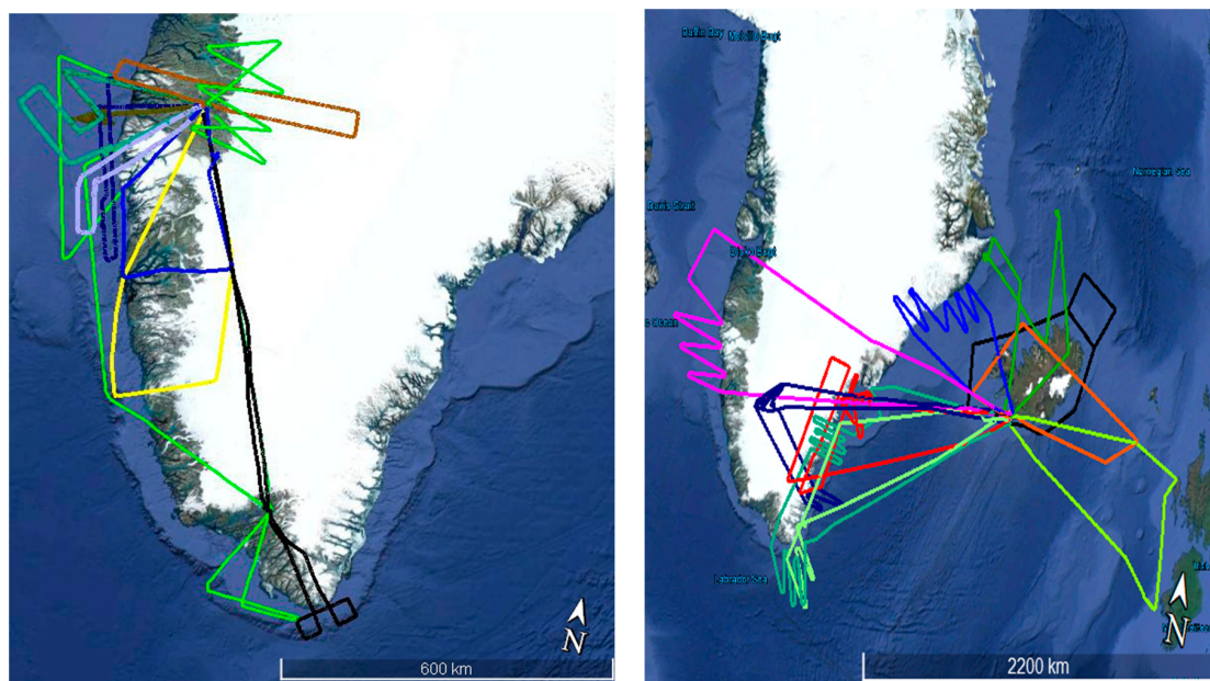
Figure 1. Mission flight paths for PW1 (left) and PW2 (right) (Google Earth).
