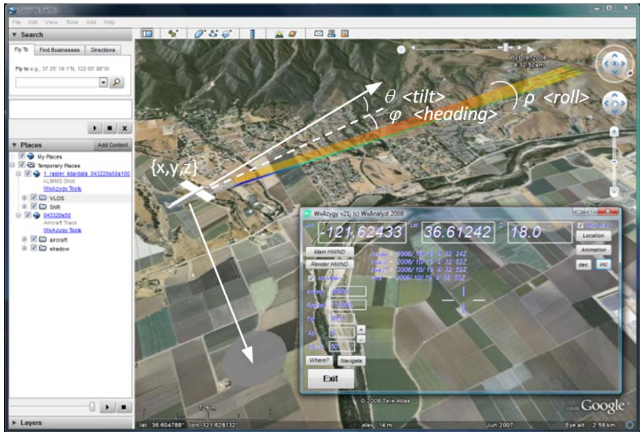
Figure 2 – Geometry of a scanning DWL profile, shown in situ from an arbitrary perspective with respect to the aircraft platform. WxAnalyz's WxAzygy™ Interactive Interface is overlaid onto Google Earth for data visualization and user control of flight data processing.
